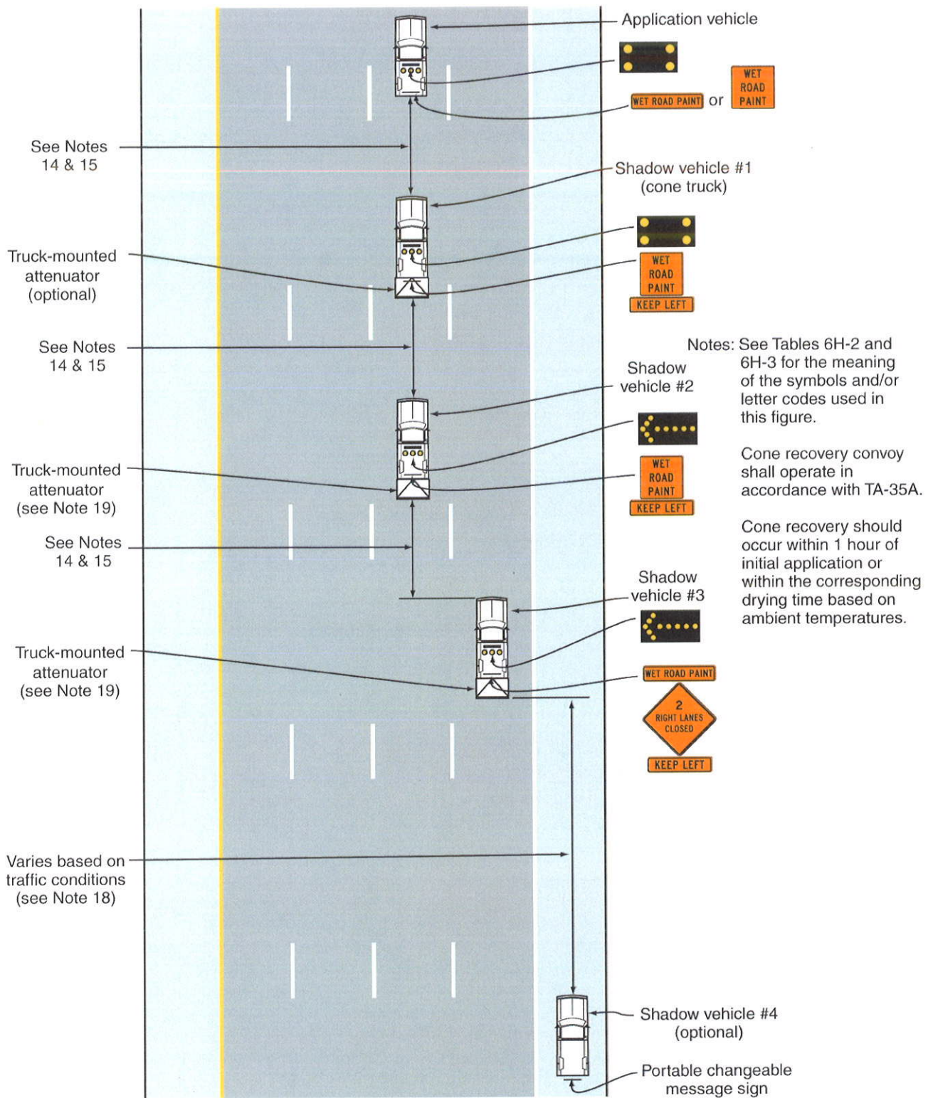
Figure 6H-35G. Mobile Striping Operations on an Interstate, Freeway, or Expressway with a Double Lane Closure and a Separate Cone Recovery Convoy (TA-35G) (Delaware Revision)
