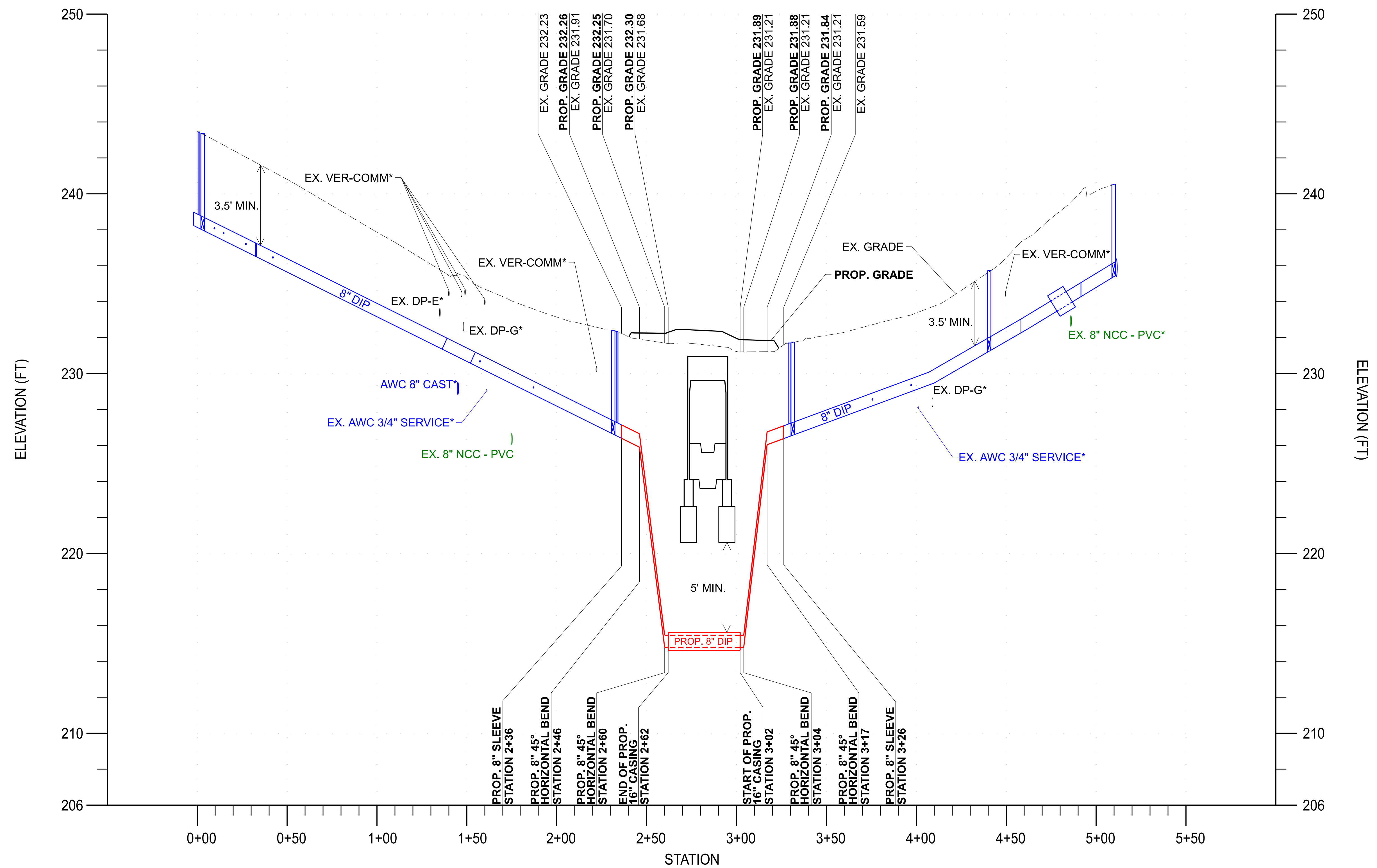
ARTESIAN WATER ALIGNMENT - 8" DIP OAK RIDGE ROAD ROAD STA. 301+86 (25' L) TO ROAD STA. 302+74 (25' L)
